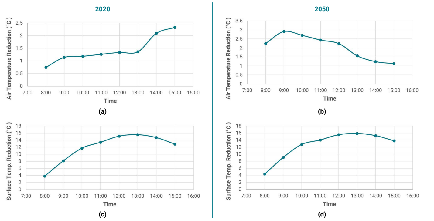
Figure 36: Maximum air temperature reductions for (a) 2020 and (b) 2050; and typical peak surface temperature reductions for (c) 2020 and (d) 2050; from the combination of all cooling interventions including water misting (Scenario 8) compared to Scenario 1
