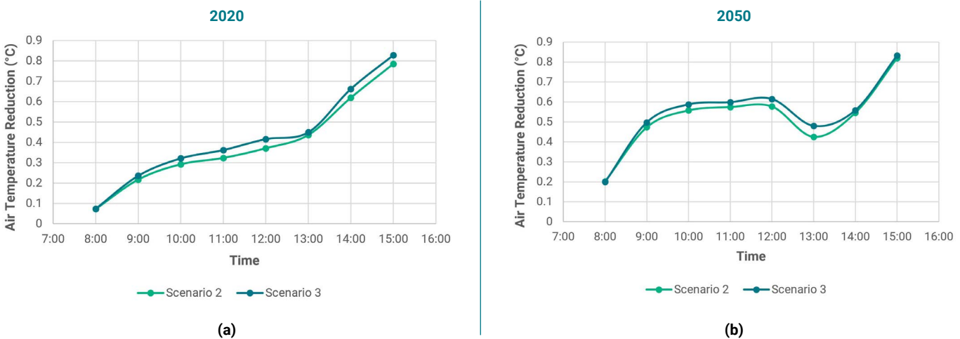
Figure 22: Maximum air temperature reductions of optimised private green coverage for all new buildings (Scenario 3) and moderate private green coverage (Scenario 2) in comparison to BAU private green coverage (Scenario 1) for (a) 2020 and (b) 2050
