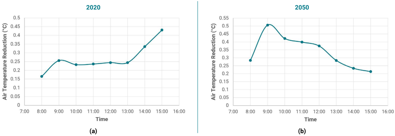
Figure 30: Maximum air temperature reductions from applying cool roofs to all existing buildings in comparison to the base case in (a) 2020 and (b) 2050
