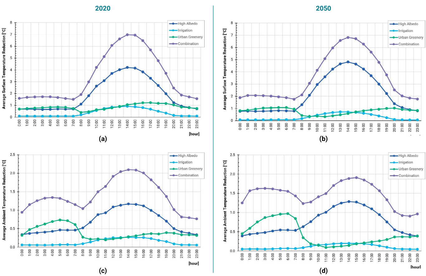
Figure 10: Comparison of the cooling intervention scenarios against the base case showing average reductions in surface temperatures for (a) 2020; and (b) 2050; and ambient temperatures for (c) 2020; and (d) 2050; averaged across February for Greater Melbourne
