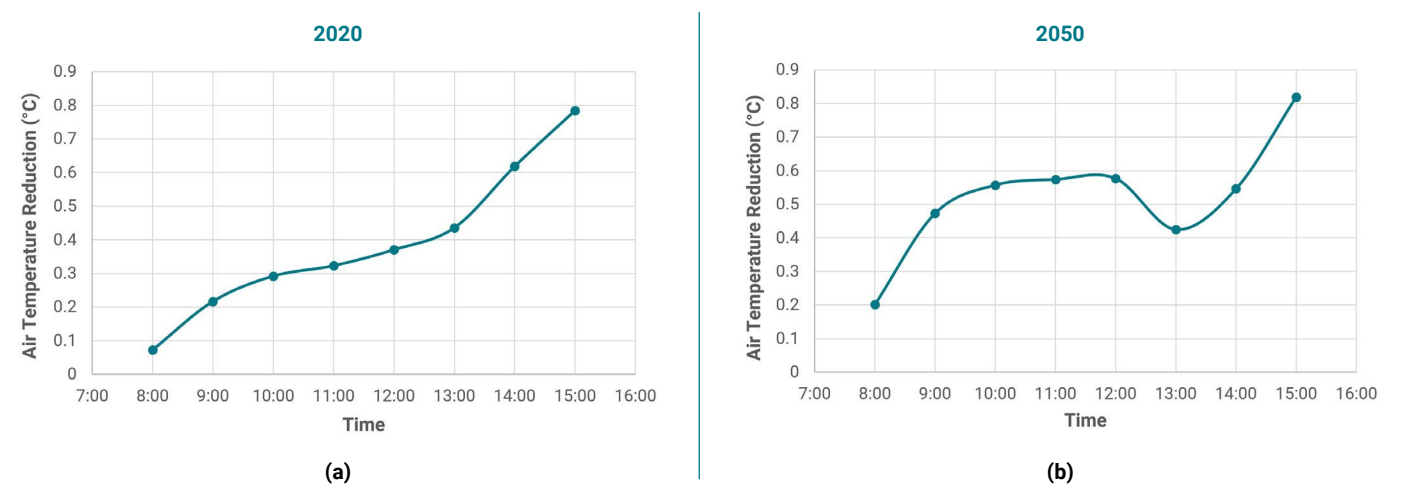
Figure 19: Maximum air temperature reductions of moderate private green coverage for all new buildings (Scenario 2) compared to BAU private green coverage (Scenario 1) for (a) 2020 and (b) 2050
