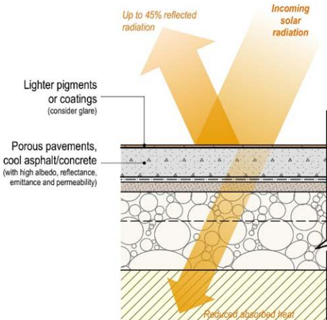
Left: Cross section through a typical cool pavement (Osmond & Sharifi, 2017)
