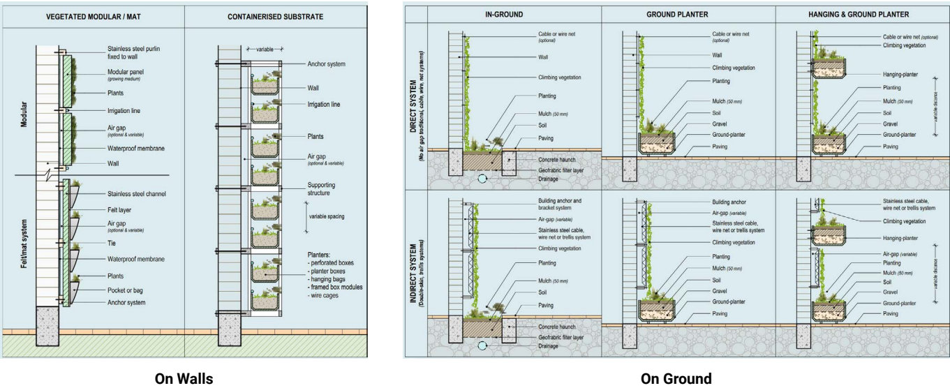
Below: Typical cross sections of vertical greenery systems (Osmond & Sharifi, 2017)
