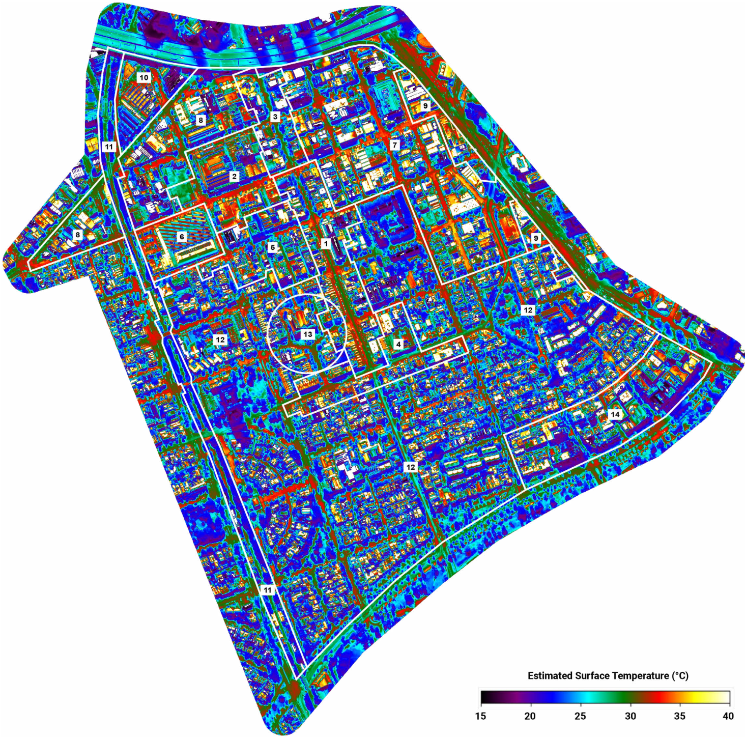
Figure 3: Airborne thermal imagery of the South Melbourne Study Area taken at approximately 13:00 on April 14, 2020
