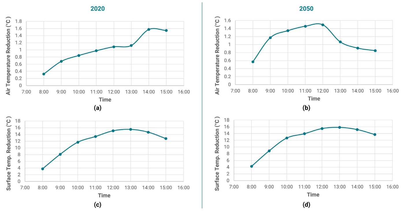
Figure 33: Maximum air temperature reductions for (a) 2020 and (b) 2050; and typical peak surface temperature reductions 6 for (c) 2020 and (d) 2050; from the combination of all cooling interventions (Scenario 7) compared to Scenario 1
