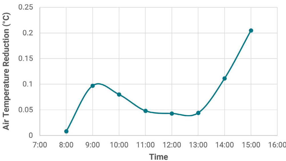
Figure 39: Average air temperature reductions from the increased building height (Scenario 9) in comparison to Scenario 2 for 2020 (Note: differences between 2020 and 2050 were negligible)
