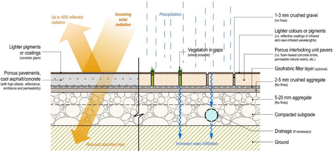
Below: Typical cross sections through cool and permeable pavements (Osmond & Sharifi, 2017)
