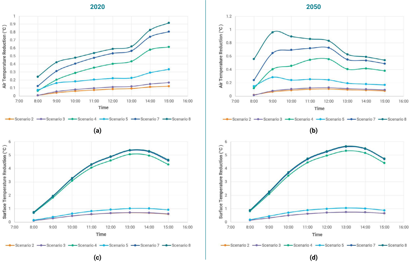
Figure 40: Intervention scenarios in comparison to Scenario 1 showing average air temperature reductions for (a) 2020 and (b) 2050; and average surface temperature reductions for (c) 2020 and (d) 2050
