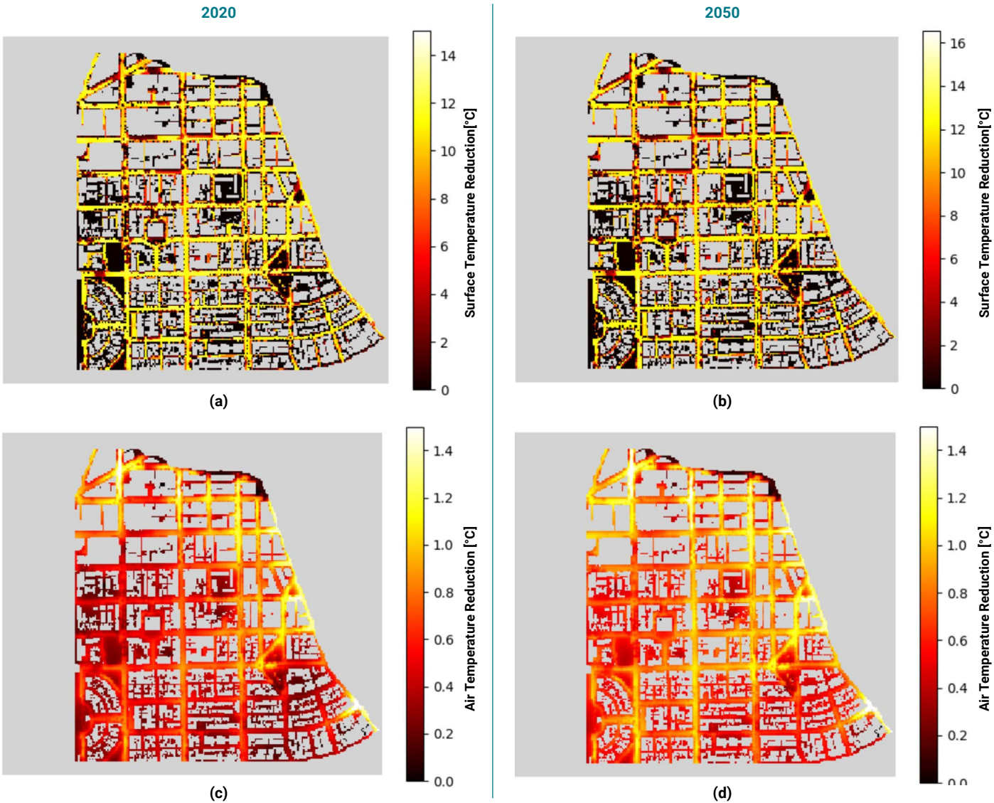
Figure 24: Surface temperature reductions for (a) 2020 and (b) 2050; and air temperature reductions for (c) 2020 and (d) 2050; from the application of cool materials (Scenario 4) compared to Scenario 1
