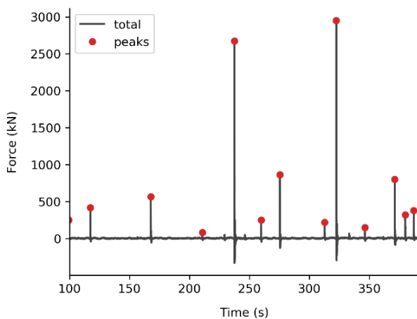
Figure 6 Identification of peak total uplift forces for Design condition 1 with 2.25 m AHD SWL
