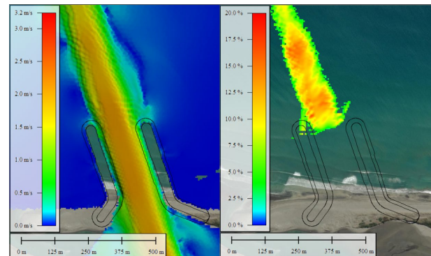
Figure 8: Example of current velocity from the TUFLOW FV model during peak velocity (left figure) and wave-current interaction in terms of percentage difference for H_s = 2\text{m} , WL = \text{MSL} during a 5% AEP river flood event during peak velocity (right figure)
