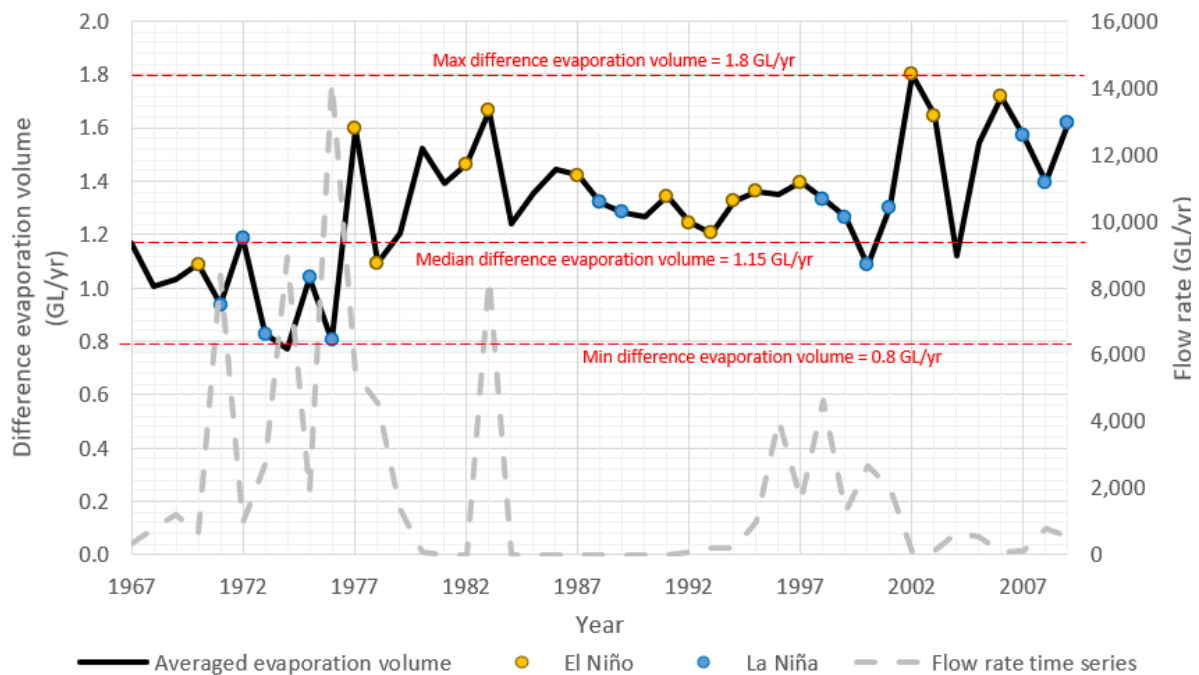
Figure ES2 Yearly difference of evaporation volume with and without the weir, plotted with annual flow.
