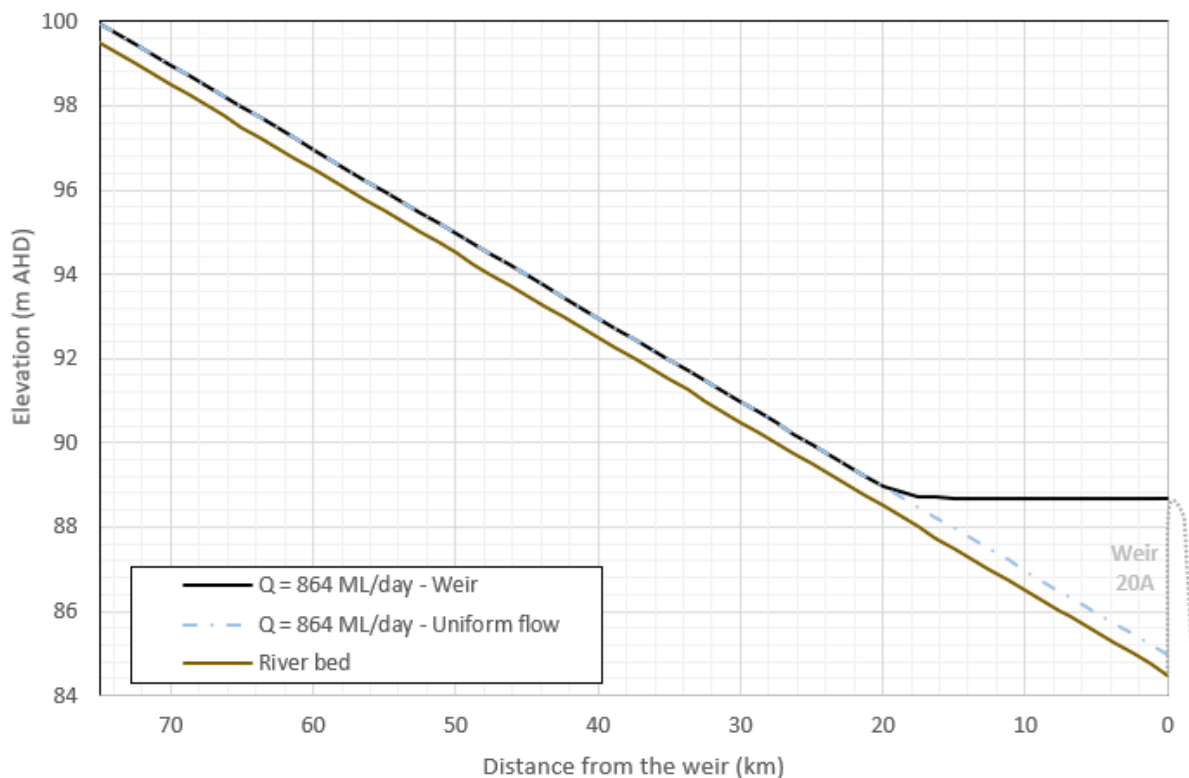
Figure 3.5 Estimated flow depths for a flow rate of 864 ML/day and a river slope of 0.02%
