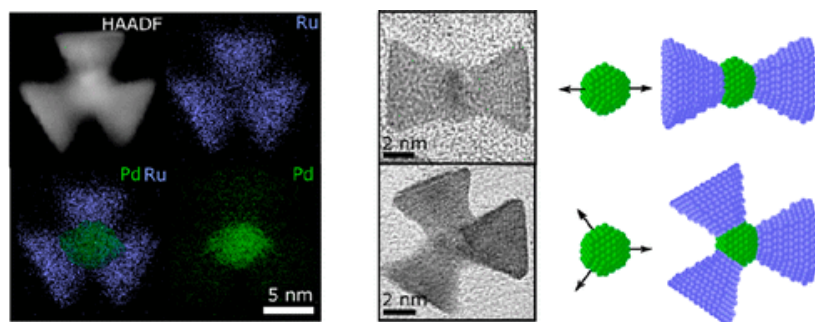
Figure 1: Energy dispersive X-ray spectroscopy elemental mapping of Pd-Ru branched nanoparticles and TEM images of individual nanoparticles. Models show the controlled direction of growth of Ru from Pd seed.
